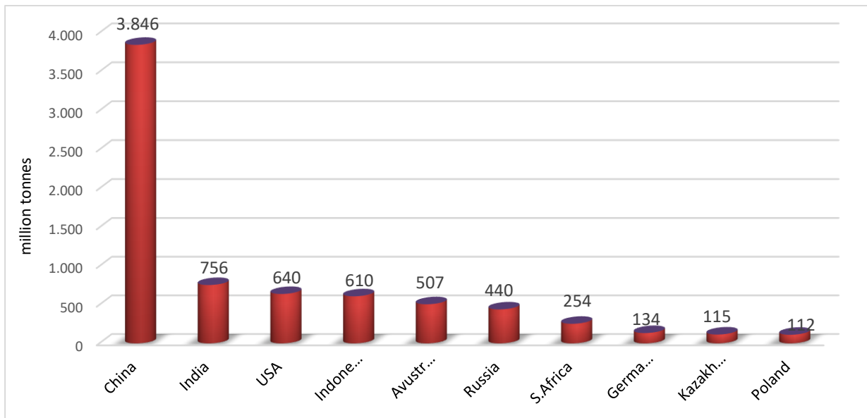
Figure 2: Coal Production in 2019 by Countries (IEA, 2020)
