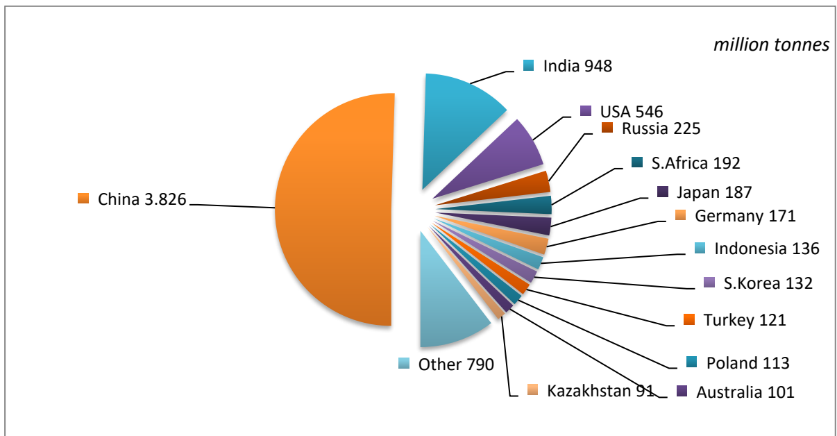
Figure 6: Coal Consumption in 2019 by Countries
