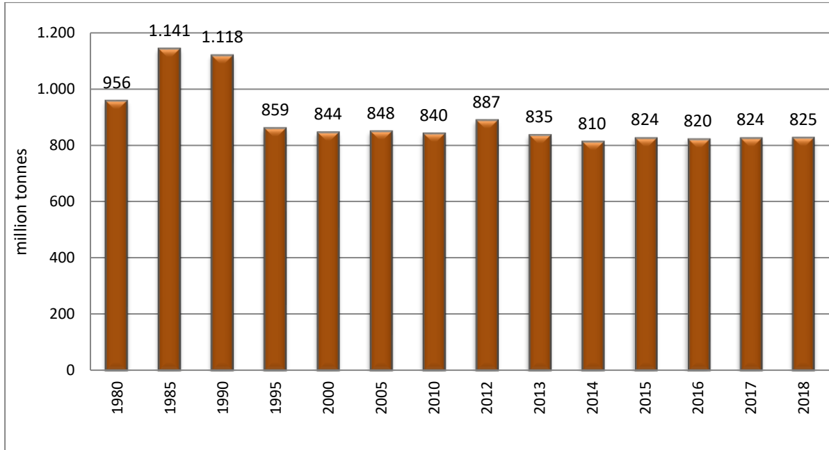
Figure 3: World Lignite Production (IEA, 2020)
