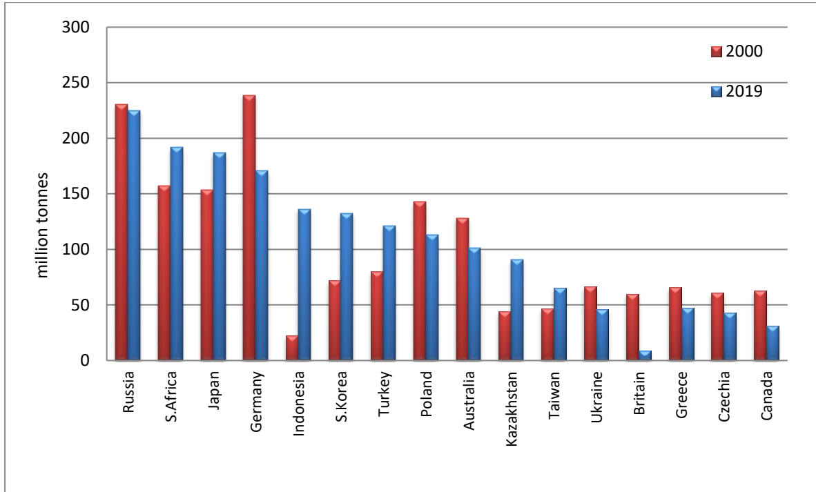
Figure 5: Change in Coal Consumption from 2000 to 2019
