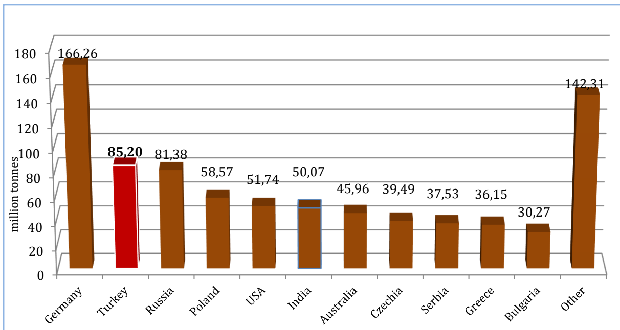
Figure 4: Lignite Production in 2018 by Countries (IEA, 2020)
