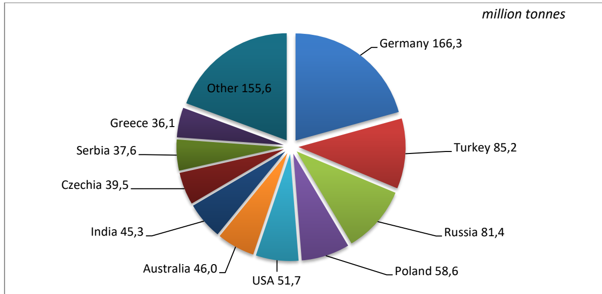
Figure 7: Lignite Consumption in 2018 by Countries
