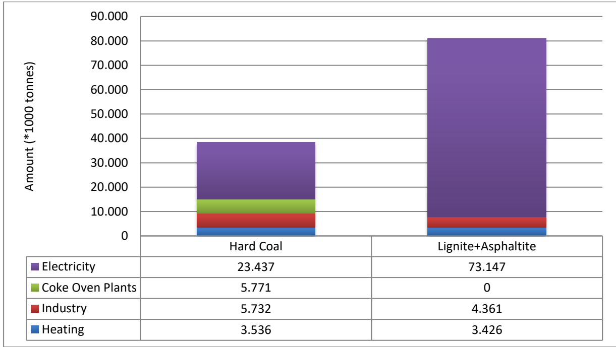
Figure 6: Consumption Distribution of Coal Supplies in 2018 by Sectors
