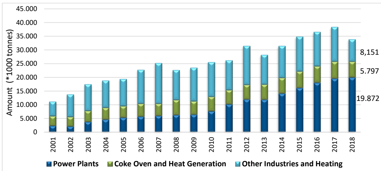
Figure 5: Consumption of Domestic and Imported Hard Coal According to Utilization Areas
